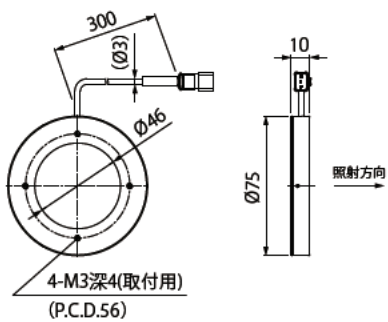
LDR-146RD2-LA1/SW2-LA1/BL2-LA1/GR2-LA1
