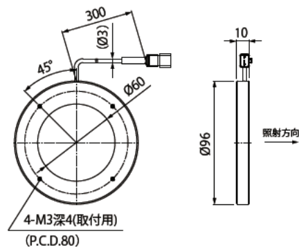
LDR-96RD2-LA1/SW2-LA1/BL2-LA1/GR2-LA1
