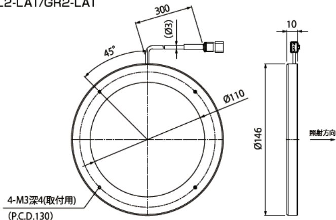
LDR-146RD2-LA1/SW2-LA1/BL2-LA1/GR2-LA1
