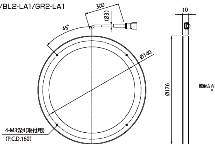
LDR-206RD2-LA1/SW2-LA1/BL2-LA1/GR2-LA1
