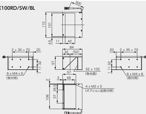
LFV3-G-100RD/SW/BL
