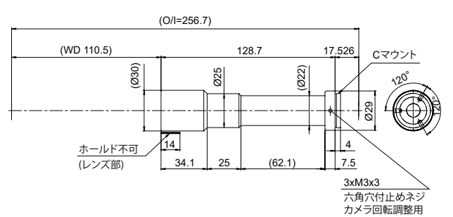
SE-110ST40-M
