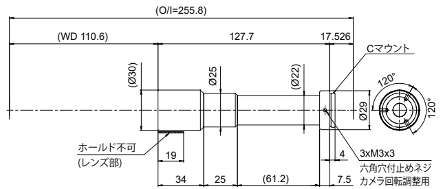
SE-110ST40-M
