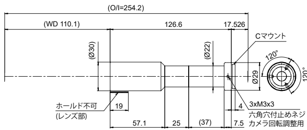
SE-110ST15-M
