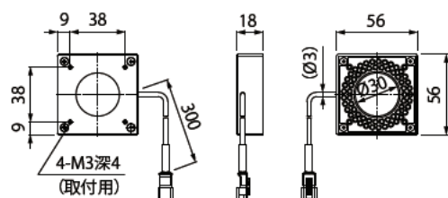
SQR-56RD2/RD2-WD
